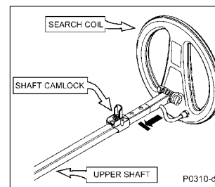
Figure 2.5 Sliding lower shaft into upper shaft
